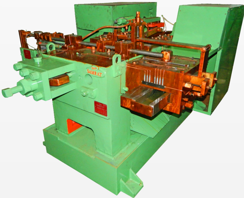
Hot Nut Header Machine
